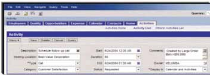
OracleBI Delivers
